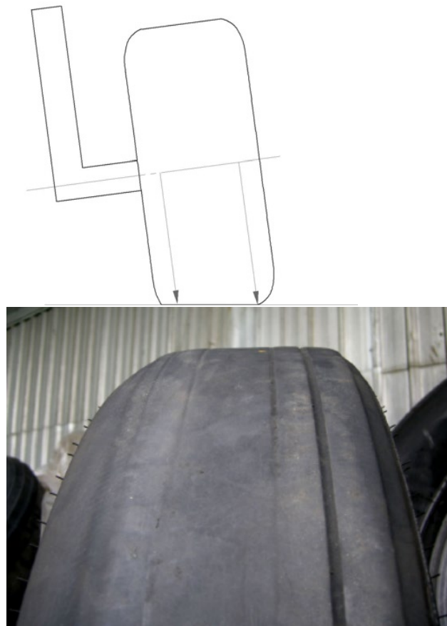
Figure 516. Camber Angle – Negative Camber
