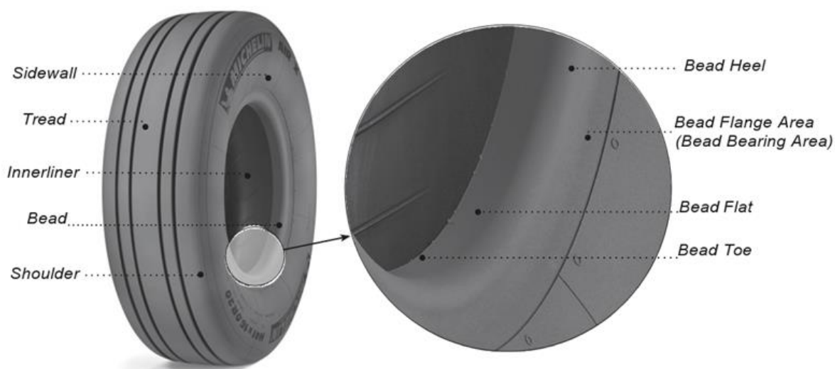
Figure 101. Tire Zones and Tire Bead Zones
